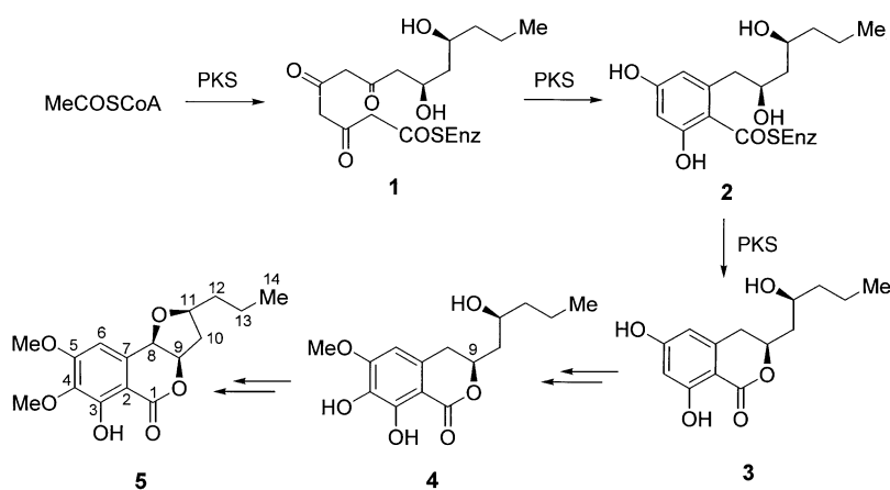
Scheme 1. Proposed biosynthesis of monocerin ( 5 ) via PKS-bound and post-assembly intermediates.
