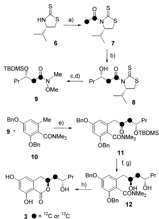
Scheme 2. Synthesis of dihydroisocoumarin 3 . Reagents and conditions: a) \text{NaN}(\text{SiMe}_3)_2 , THF, -78^\circ\text{C} ; then \text{MeCO}_2\text{COCMe}_3 , 5 h, 35%; b) \text{Sn}(\text{OTf})_2 , 1-ethylpiperidine, \text{CH}_2\text{Cl}_2 , -40^\circ\text{C} , 4.5 h; then butanal, -78^\circ\text{C} , 20 min, 88%; c) \text{Et}_3\text{N} , \text{MeNHOMe} , \text{CH}_2\text{Cl}_2 , 25^\circ\text{C} , 72 h, 92%; d) \text{TBDMSOTf} , 2,6-lutidine, \text{CH}_2\text{Cl}_2 , -25^\circ\text{C} , 1 h; then -25^\circ\text{C} \rightarrow \text{RT} , 12 h, 98%; e) \text{sec-BuLi} , THF, -72^\circ\text{C} , 15 min; then 9 , -72^\circ\text{C} , 1.25 h, 45%; f) \text{HCl}/\text{EtOH} (1%), 25^\circ\text{C} , 5 h, 87%; g) \text{AcOH} , \text{Me}_4\text{N-B}(\text{OAc})_3\text{H} , MeCN, 6.25 h, -10^\circ\text{C} , 92%; h) 3 N \text{HCl}/\text{dioxane} (1:1), reflux, 48 h, 83%. Bn = benzyl, TBDMS = tert -butyldimethylsilyl, Tf = triflate = trifluoromethanesulfonyl, THF = tetrahydrofuran.
