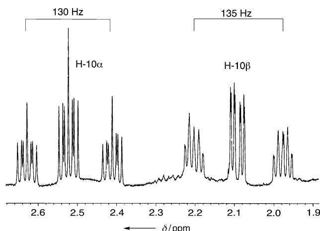
Figure 1. 600 MHz 1 H NMR spectrum showing the 10-H 2 signals of monocerin ( 5 ) enriched from incorporation of [9,10- 13 C 2 ]-labeled dihydroisocoumarin 3 .
